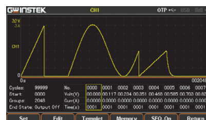
Output Waveform of the GPP-6030/3060
