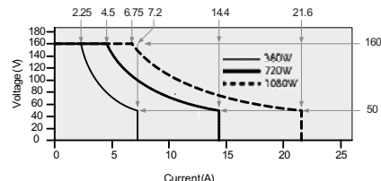
PSW 160V Series Operating Area
