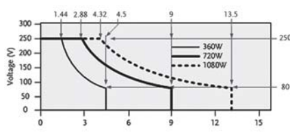
PSW 250V Series Operating Area
