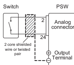
External Switch Control of the Output On/Off
