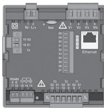
Rear view
