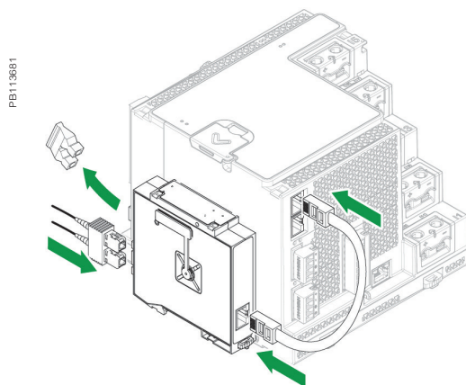
PowerLogic™ ION9000 connected with Fiber-Ethernet
