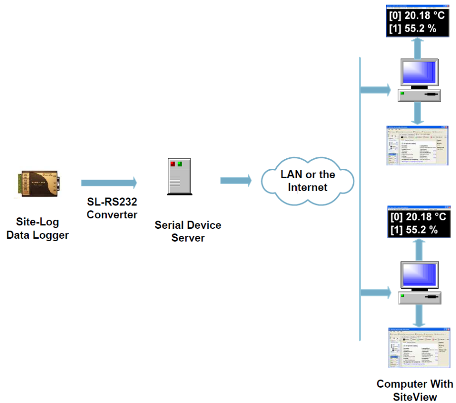
Ethernet Connection (with Ethernet – Serial Converter)
