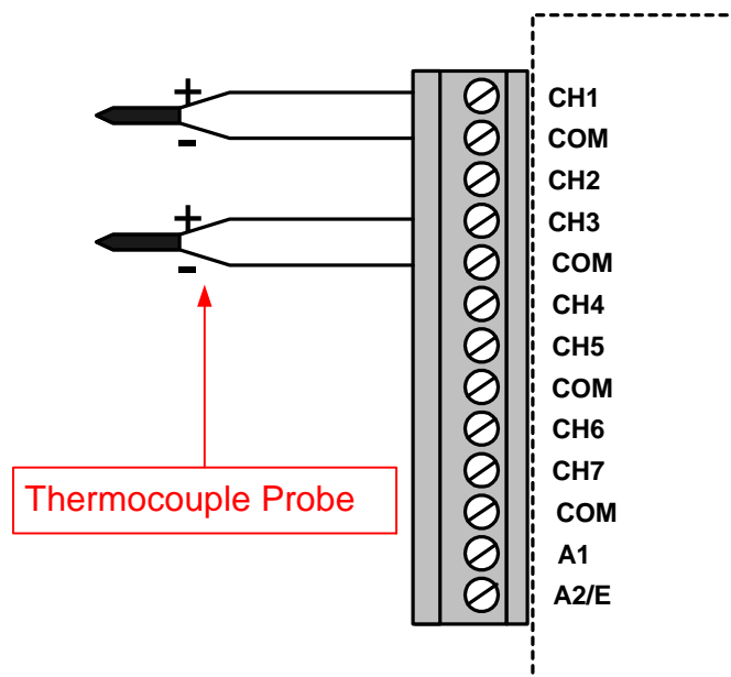
Thermocouple Input Connections
